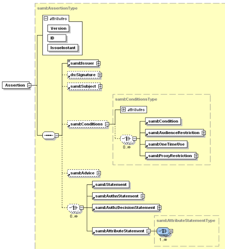
Figure 16: Identity Assertion – Top Level Elements of a SAML Assertion
