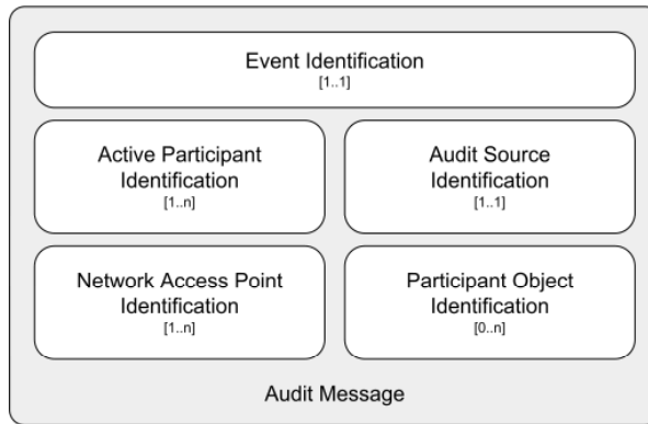
Figure 15: RFC3881 overview
