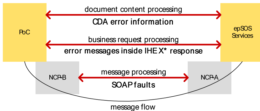
Figure 7: epSOS error handling
