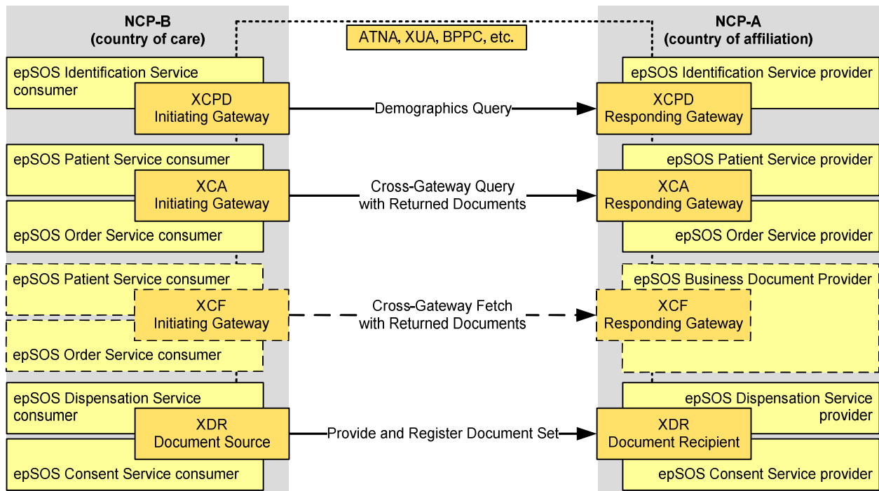
Figure 6: IHE actors and transactions that are profiled by epSOS
